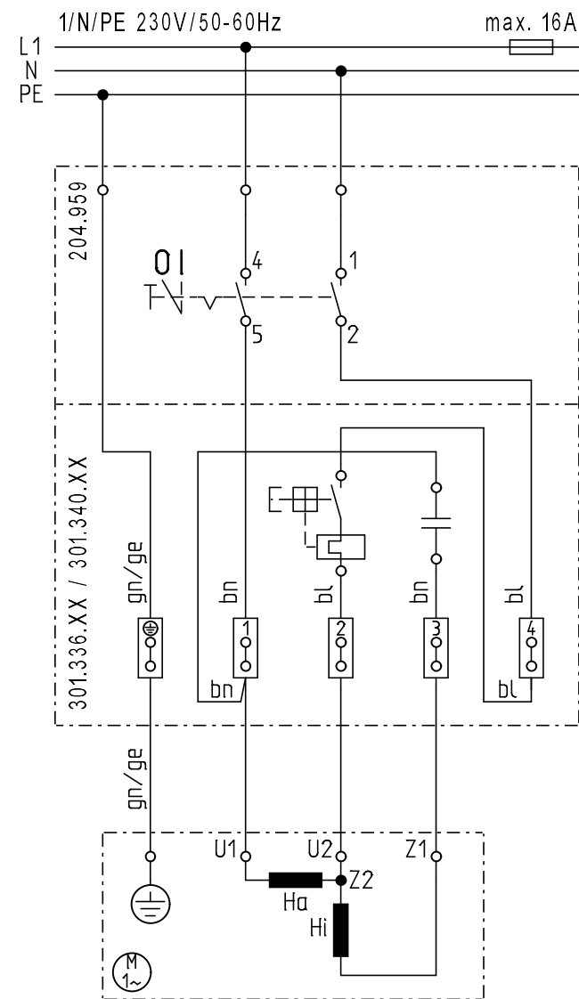
Motorschalter/motor switch 204.959 und/and Zubehör/Option 301.336.XX oder/or 301.340.XX
