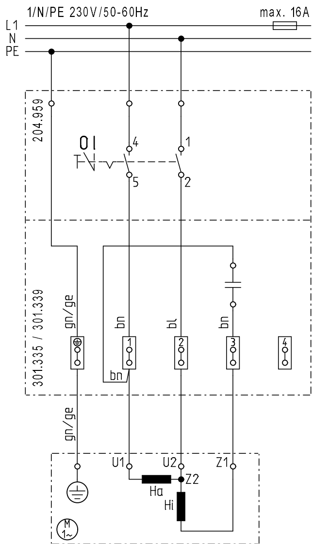
Motorschalter/motor switch 204.959 und/and Zubehör/Option 301.335 oder/or 301.339
