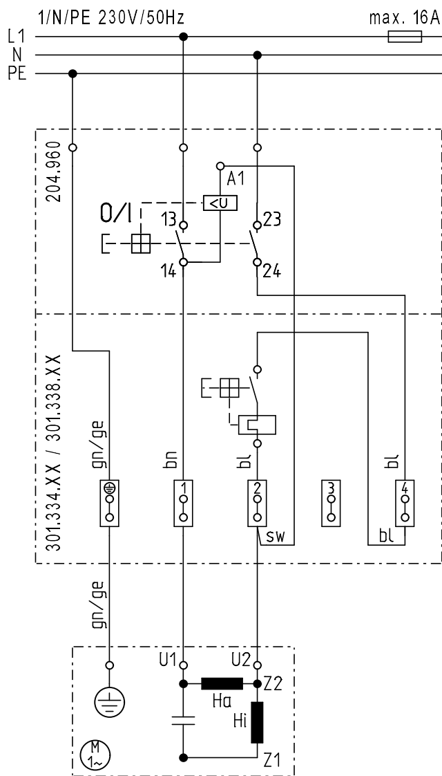
Motorschalter/motor switch 204.960 und/and Zubehör/Option 301.334.XX oder/ or 301.338.XX
