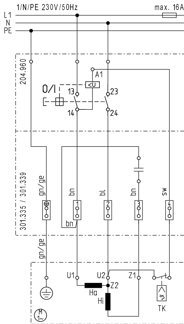
Motorschalter/motor switch 204.960 und/and Zubehör/Option 301.335 oder/ or 301.339
