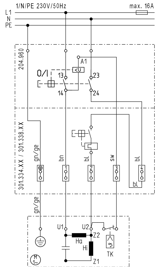
Motorschalter/motor switch 204.960 und/and Zubehör/Option 301.334.XX oder/ or 301.338.XX
