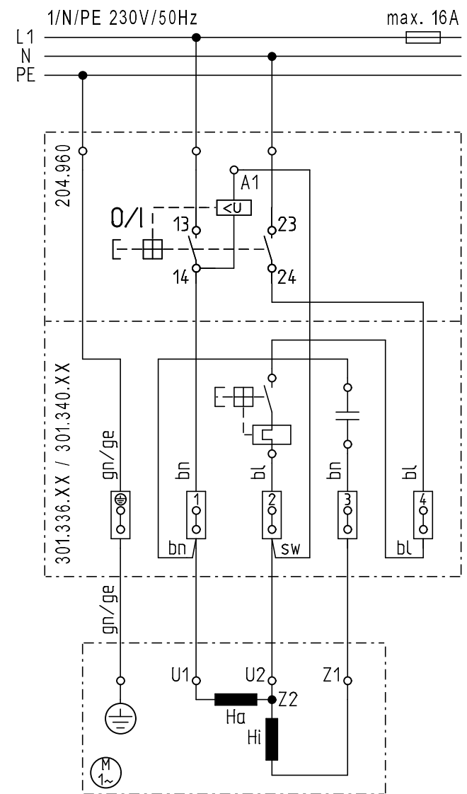
Motorschalter/motor switch 204.960 und/and Zubehör/Option 301.336.XX oder/ or 301.340.XX
